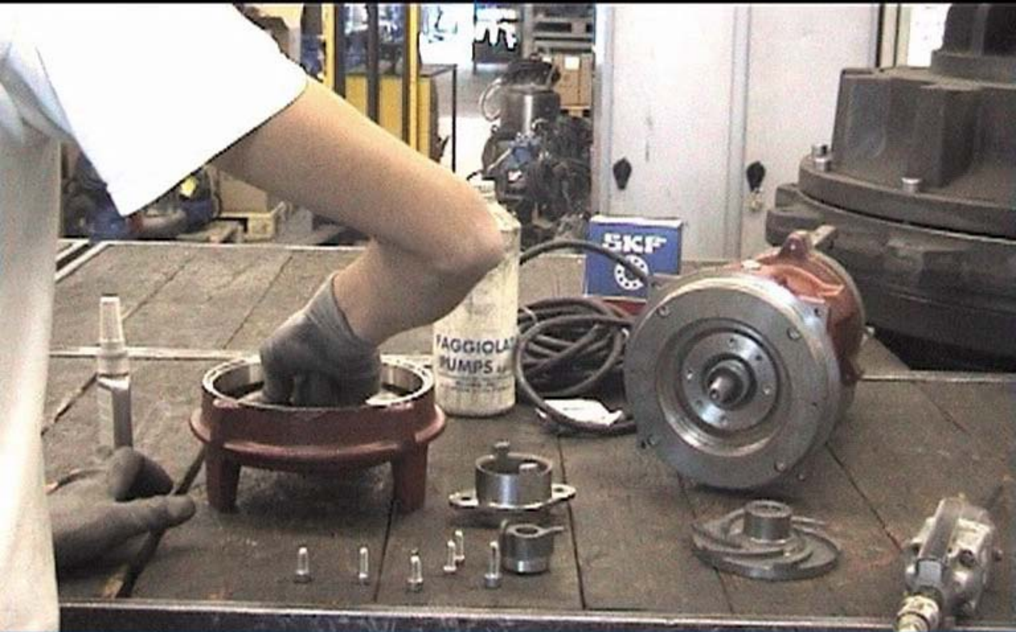
Pre assemblaggio parti idrauliche Pre-assembling of the hydraulic components
